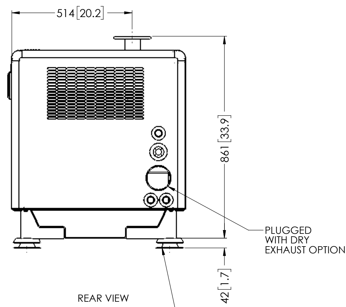
REAR VIEW
