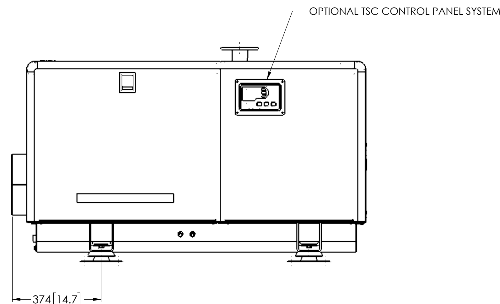
LEFT (SERVICE) SIDE VIEW
