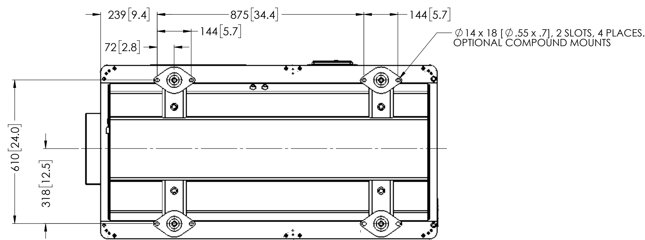
BOTTOM VIEW
