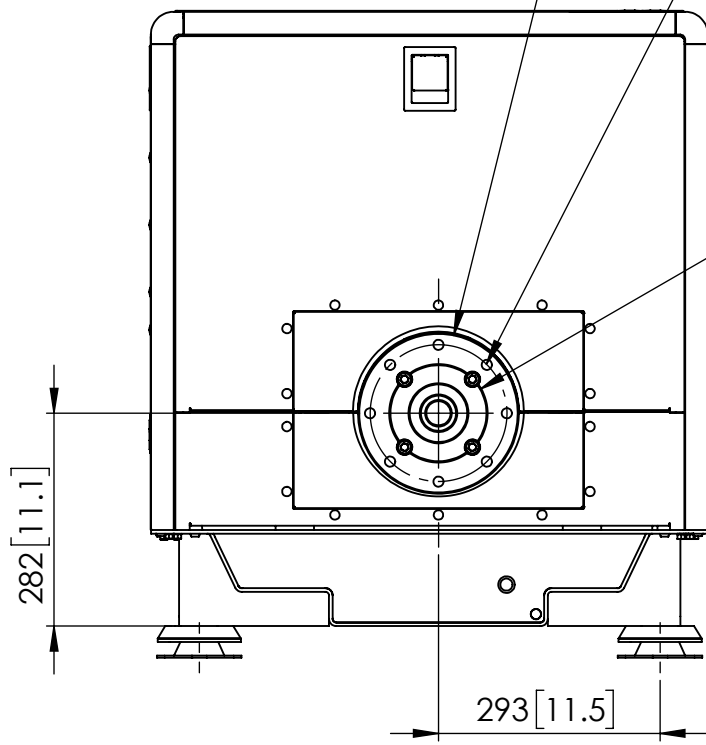
FRONT VIEW
