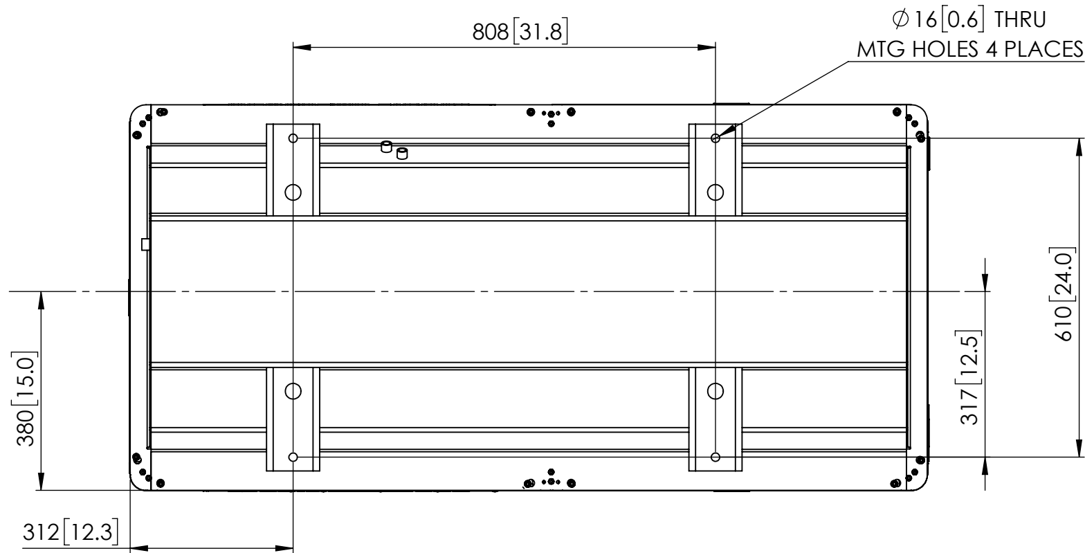
BOTTOM VIEW
