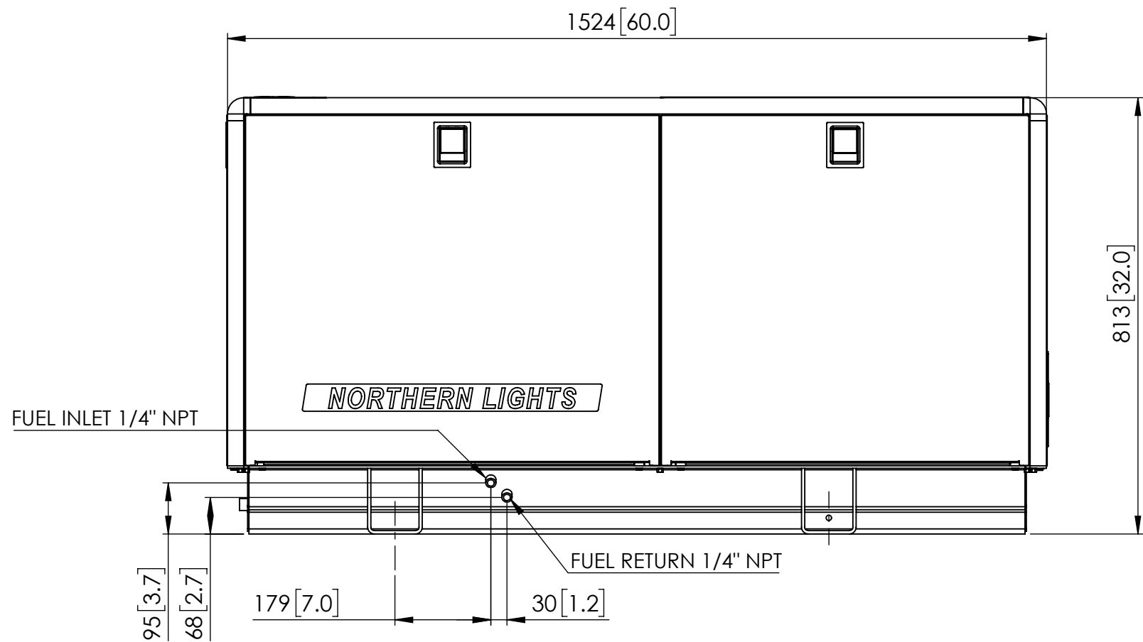
LEFT (SERVICE) SIDE VIEW
