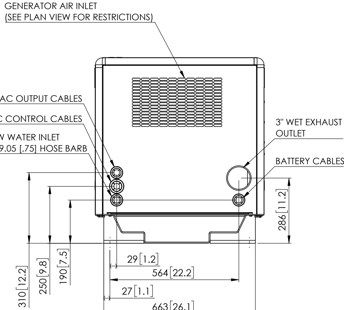
REAR VIEW
