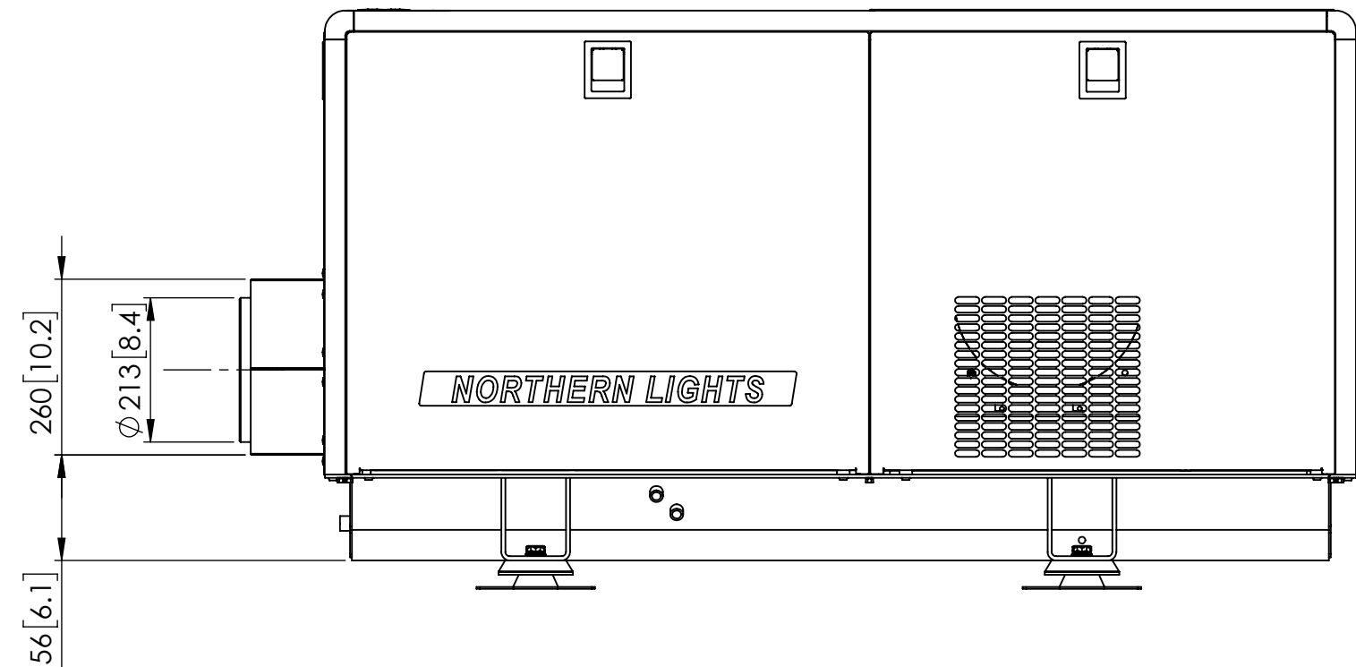
LEFT (SERVICE) SIDE VIEW
