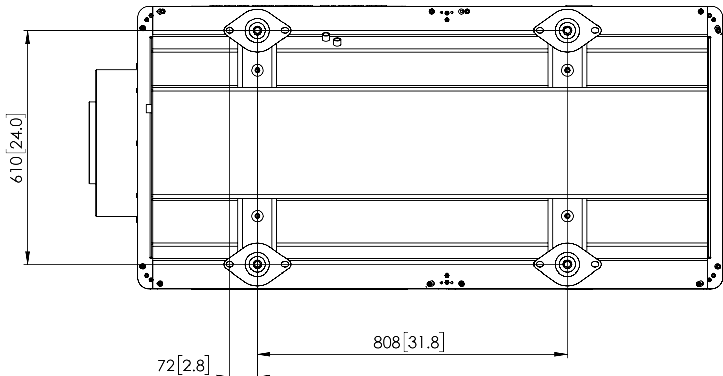
BOTTOM VIEW
