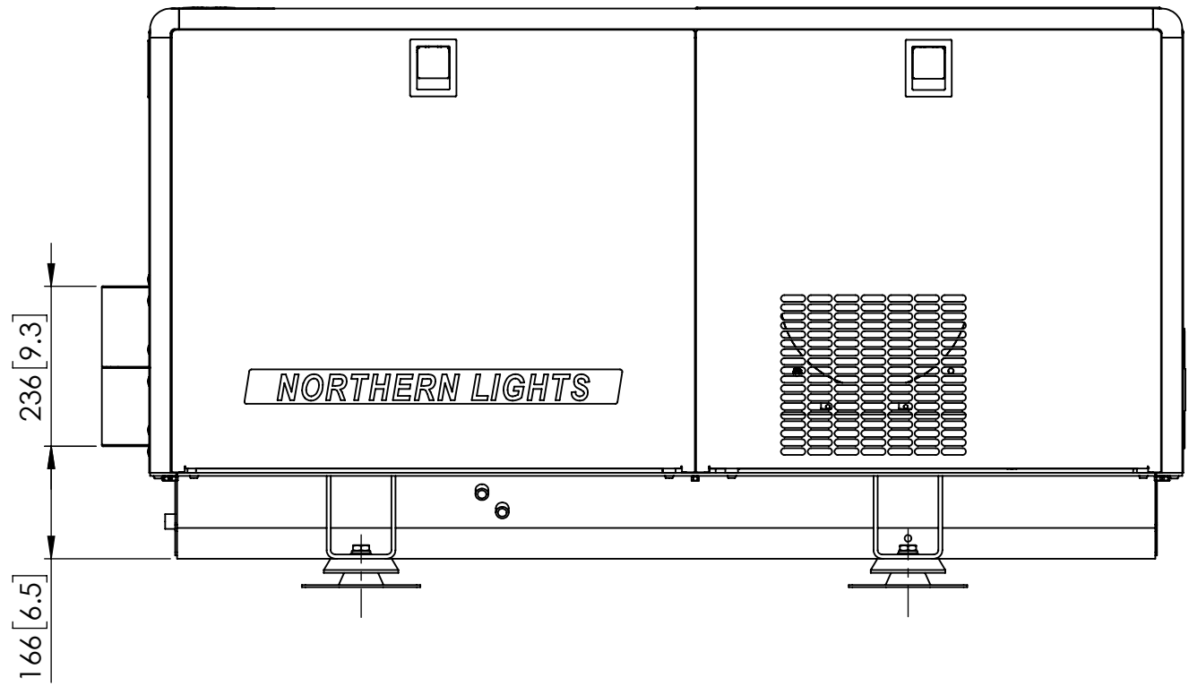
LEFT (SERVICE) SIDE VIEW
