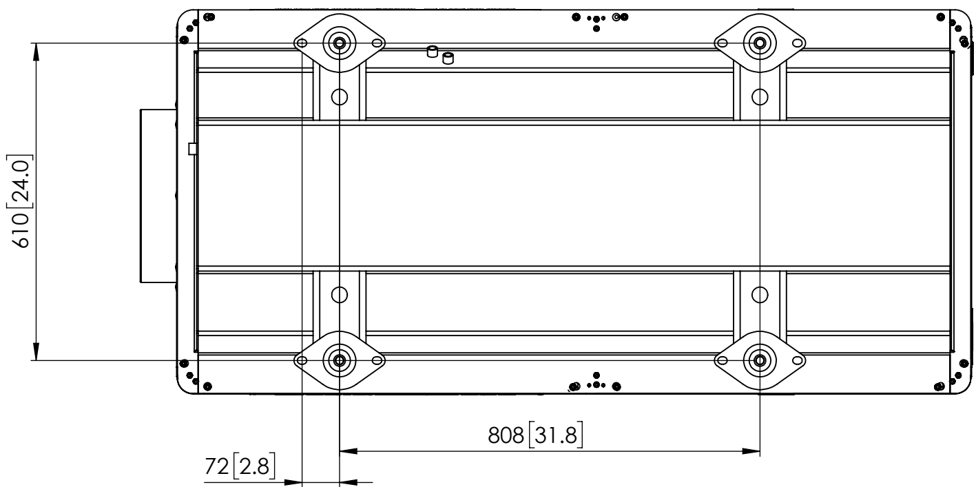
BOTTOM VIEW
