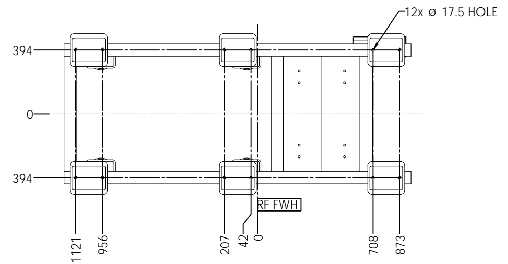
COMPOUND MOUNT BOLT PATTERN
