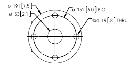
OPTIONAL DRY EXHAUST ELBOW DETAIL
