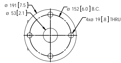
EXHAUST ELBOW DETAIL
