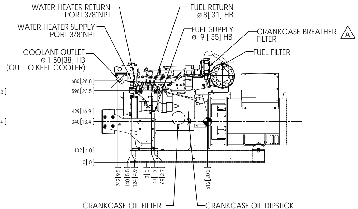
LEFT SIDE (SERVICE SIDE)
