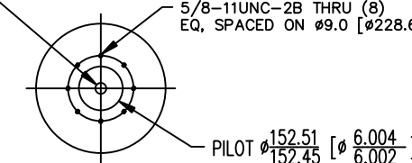
SAE D-PAD DETAIL C
