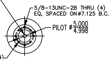
SAE C-PAD DETAIL A
