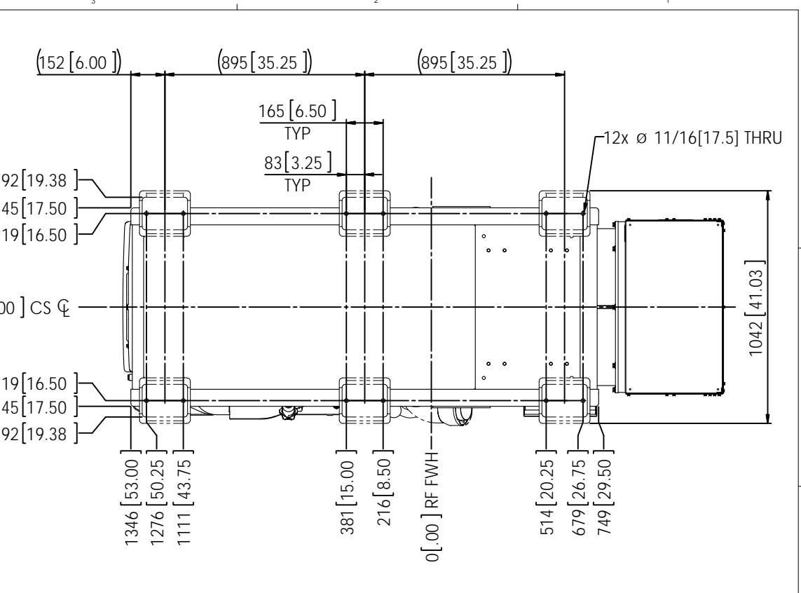
OPTIONAL COMPOUND MOUNT BOLT PATTERN
