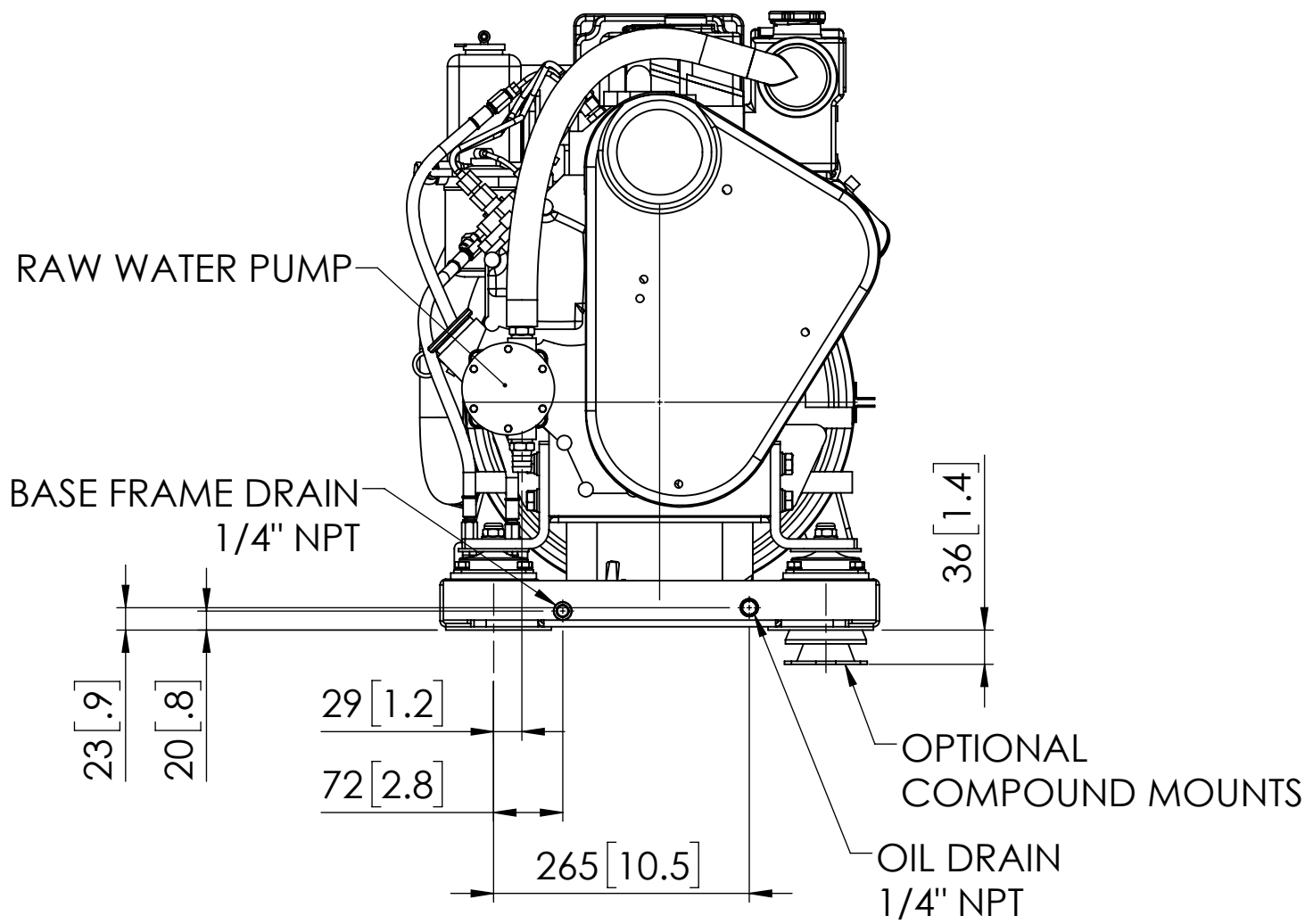
FRONT VIEW
