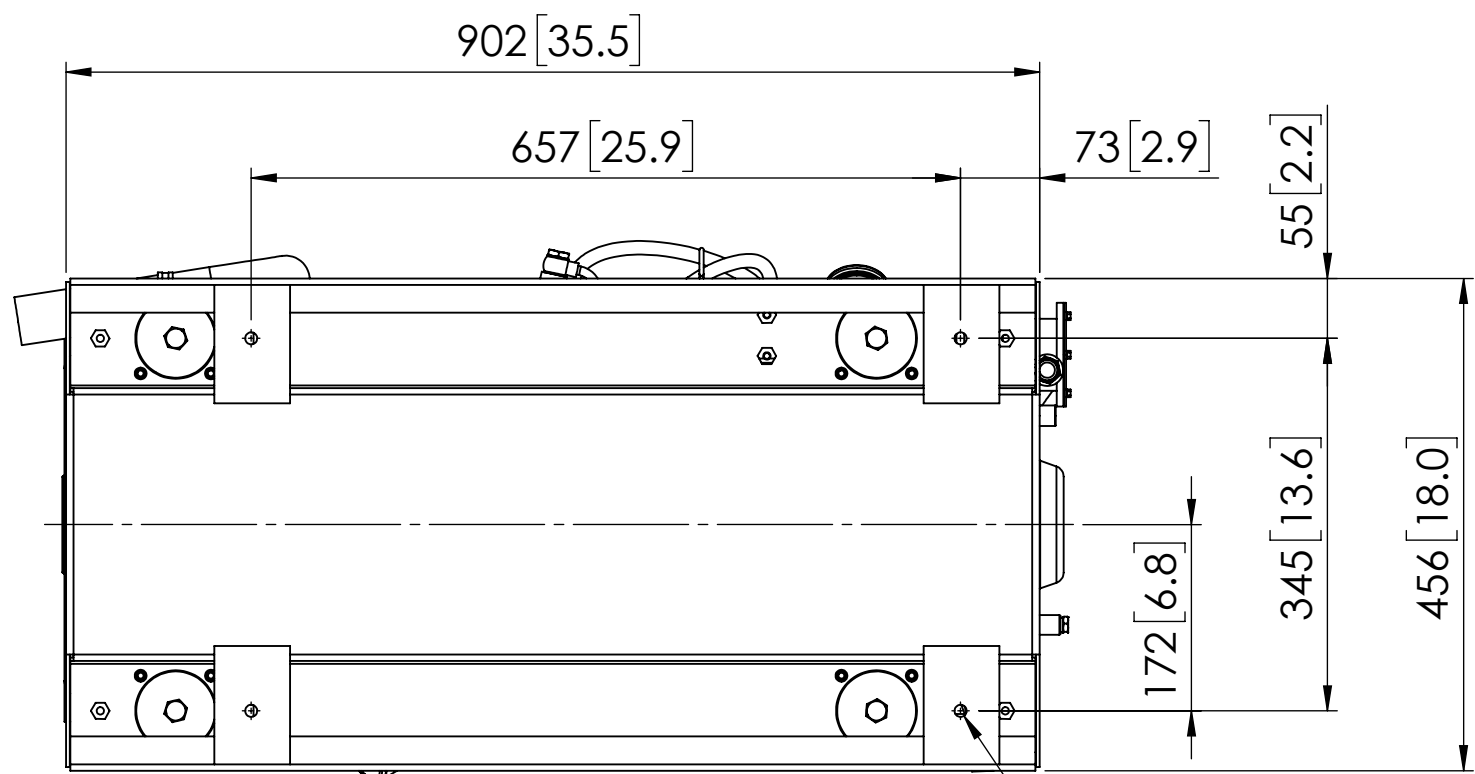
BOTOM VIEW
