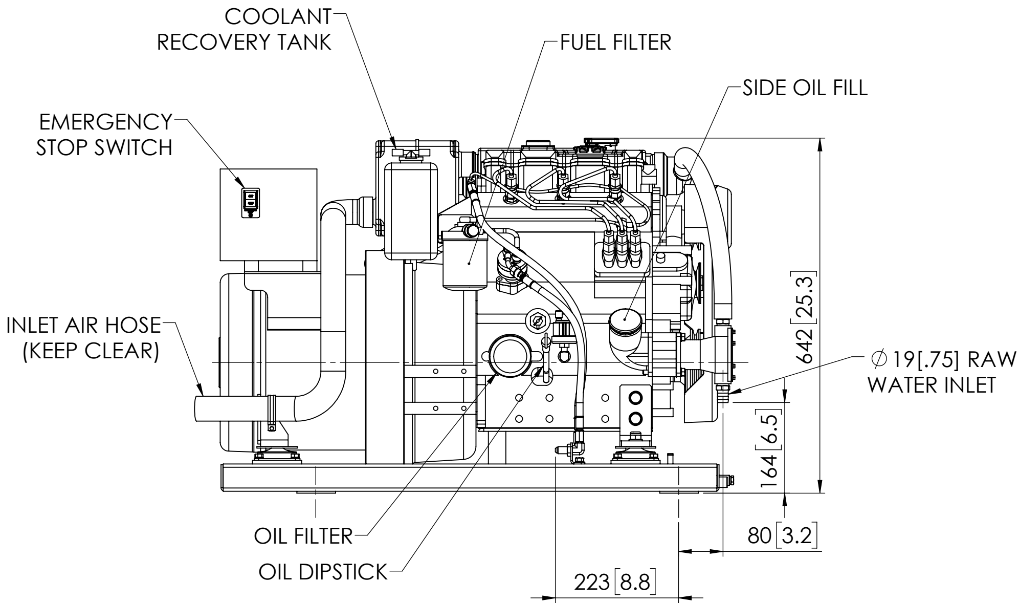
RIGHT (SERVICE) SIDE VIEW
