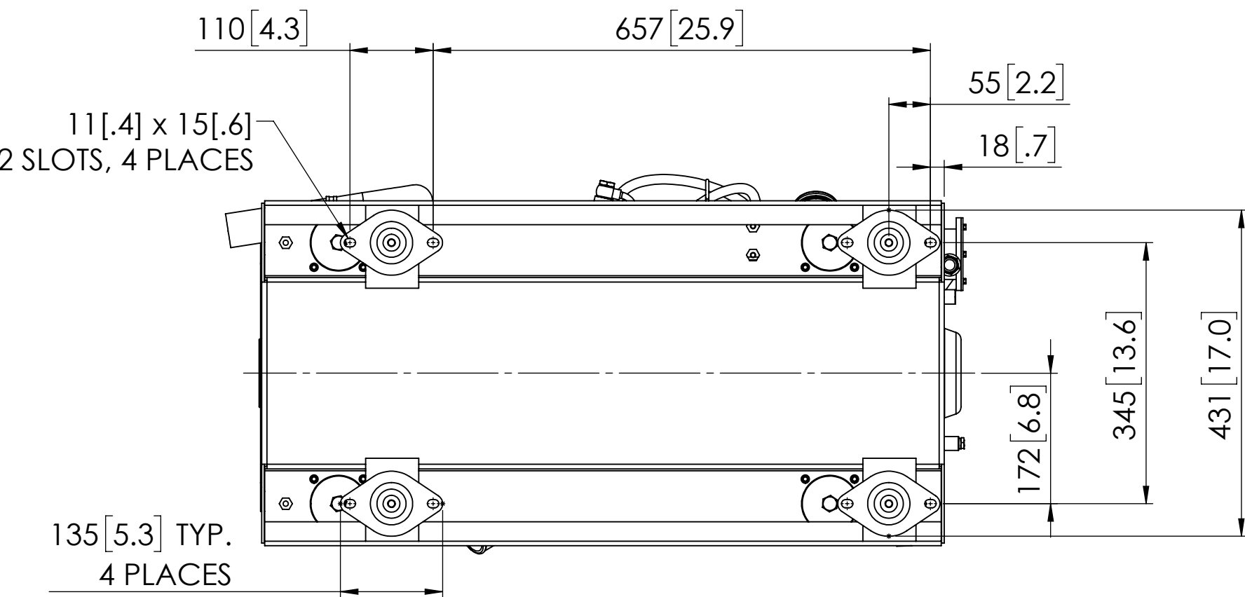
OPTIONAL COMPOUND MOUNTS
