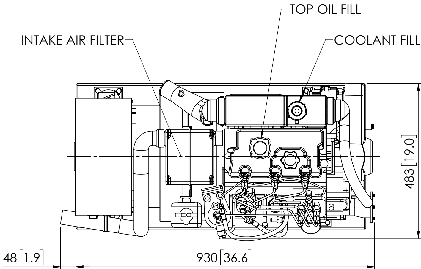
PLAN VIEW
