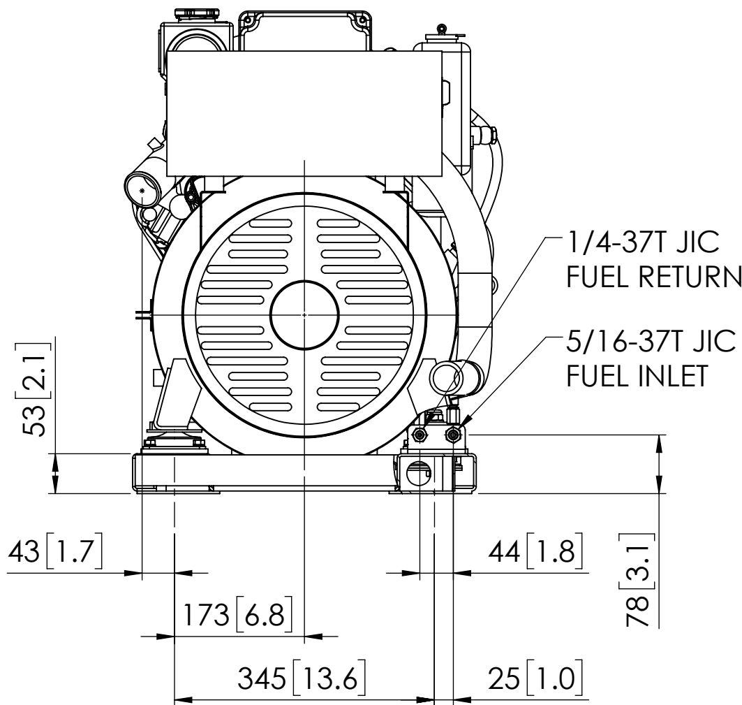
REAR VIEW
