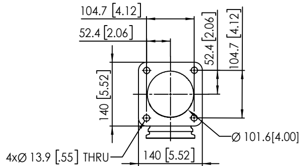
OPTIONAL DRY EXHAUST ELBOW FLANGE DETAIL
