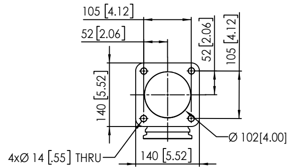
OPTIONAL DRY EXHAUST ELBOW FLANGE DETAIL
