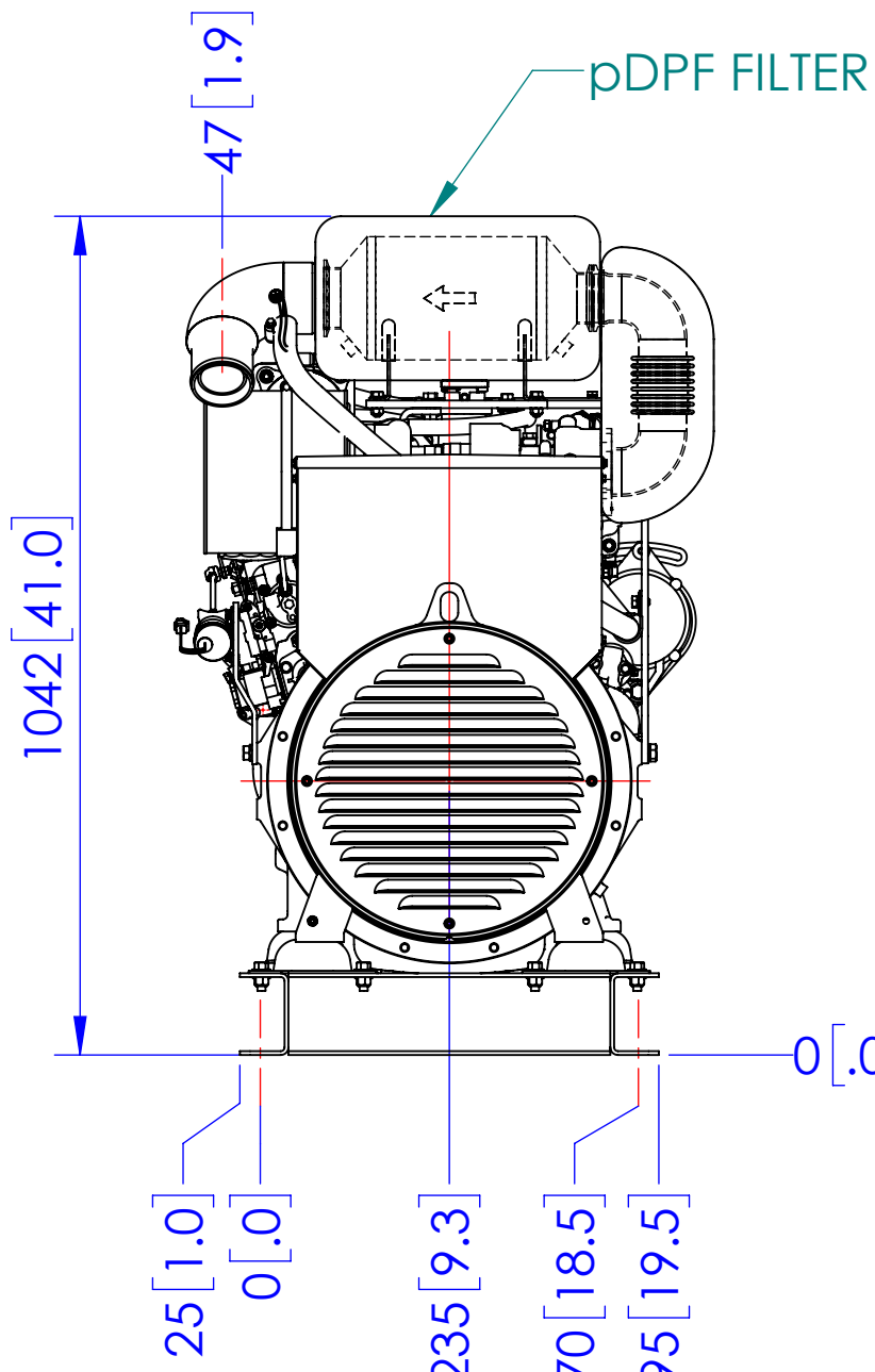
REAR
