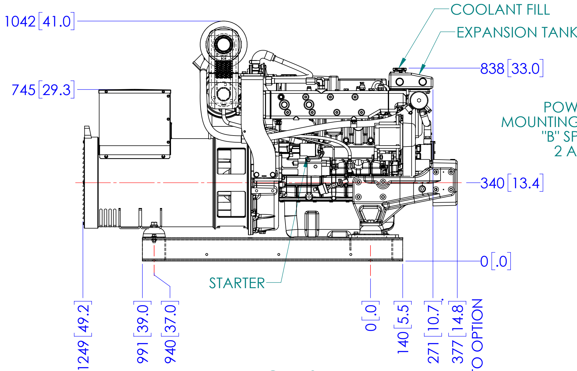
RIGHT SIDE
