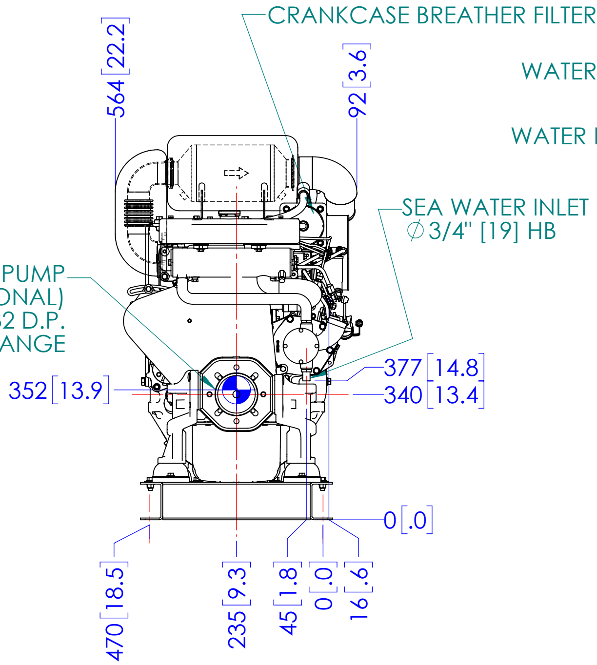
FRONT
