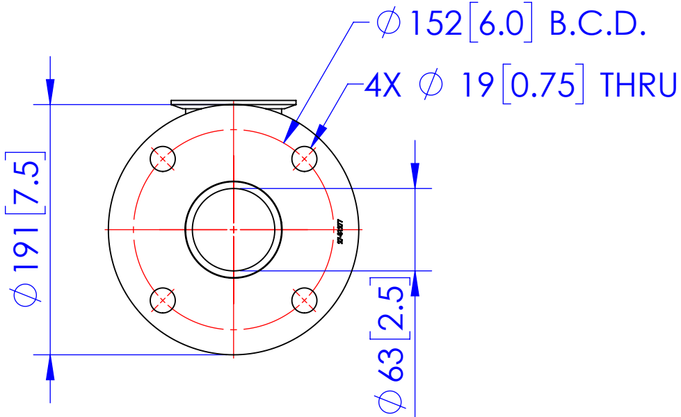
DRY EXHAUST ELBOW DETAIL SCALE 1:4
