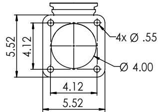
OPTIONAL DRY EXHAUST ELBOW SCALE 1:4
