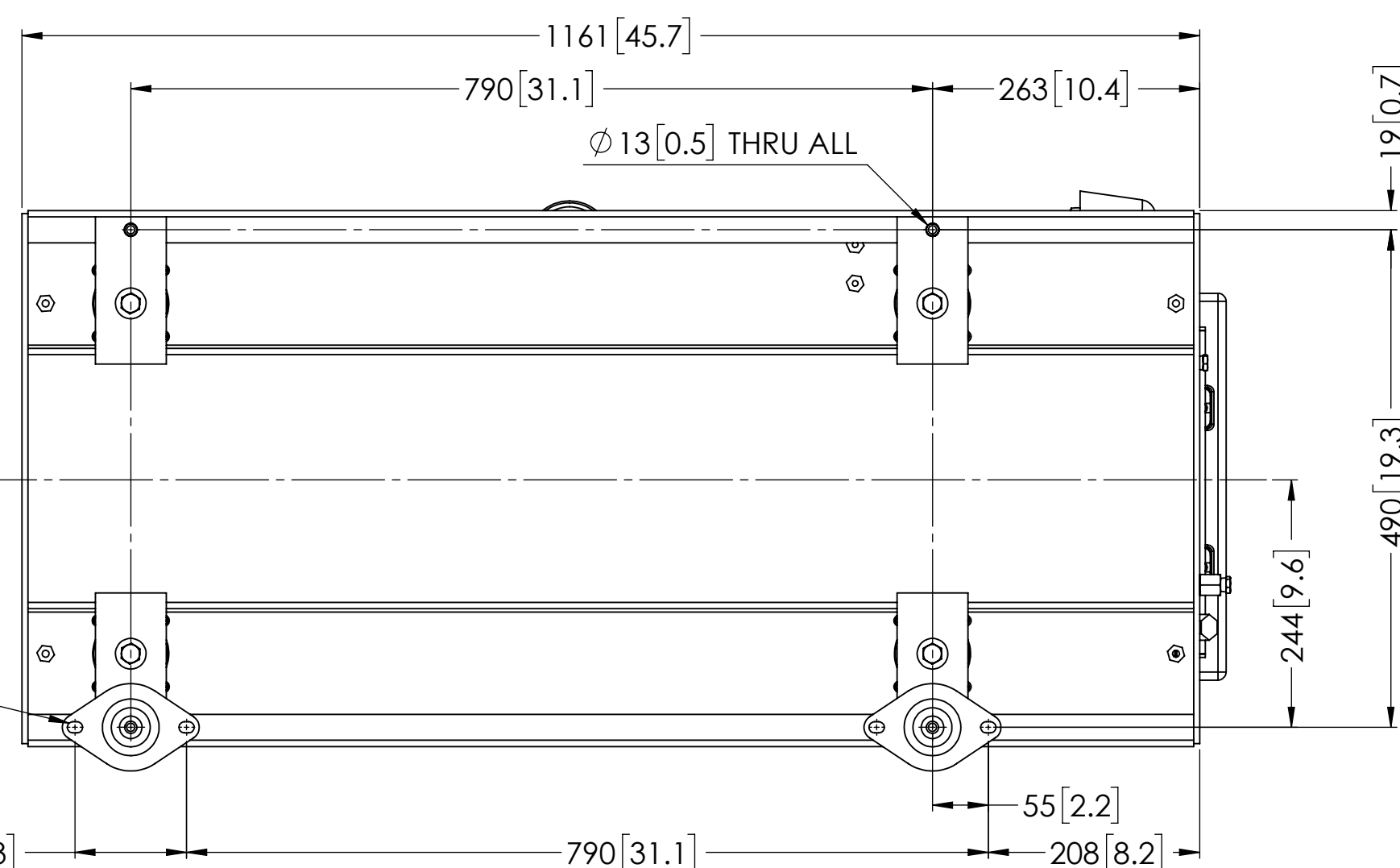
BOTTOM VIEW
