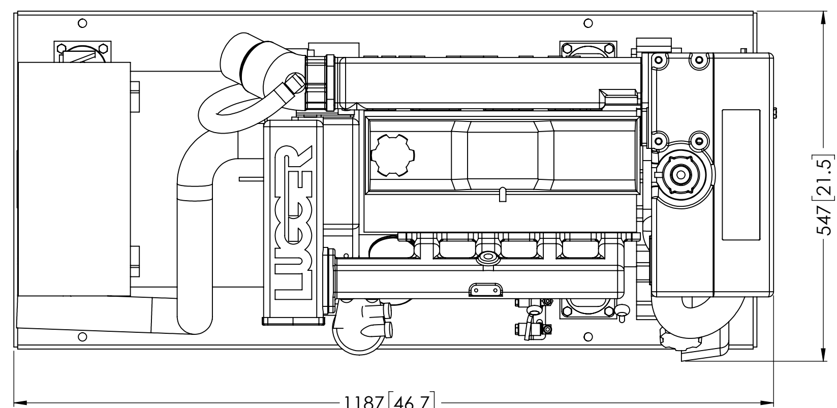
PLAN VIEW
