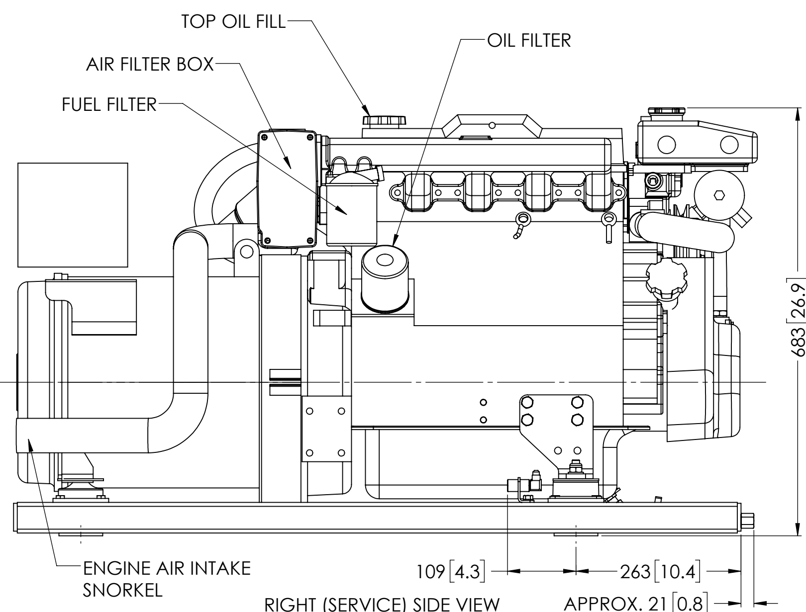
RIGHT (SERVICE) SIDE VIEW
