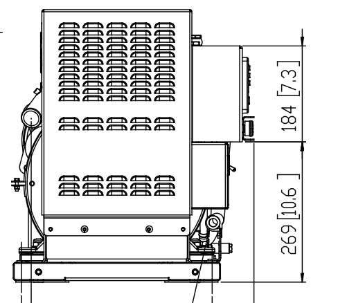
REAR VIEW
