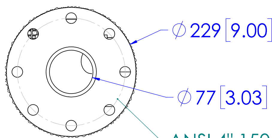
DETAIL A OPTIONAL DRY EXHAUST FLANGE SCALE 1 : 4
