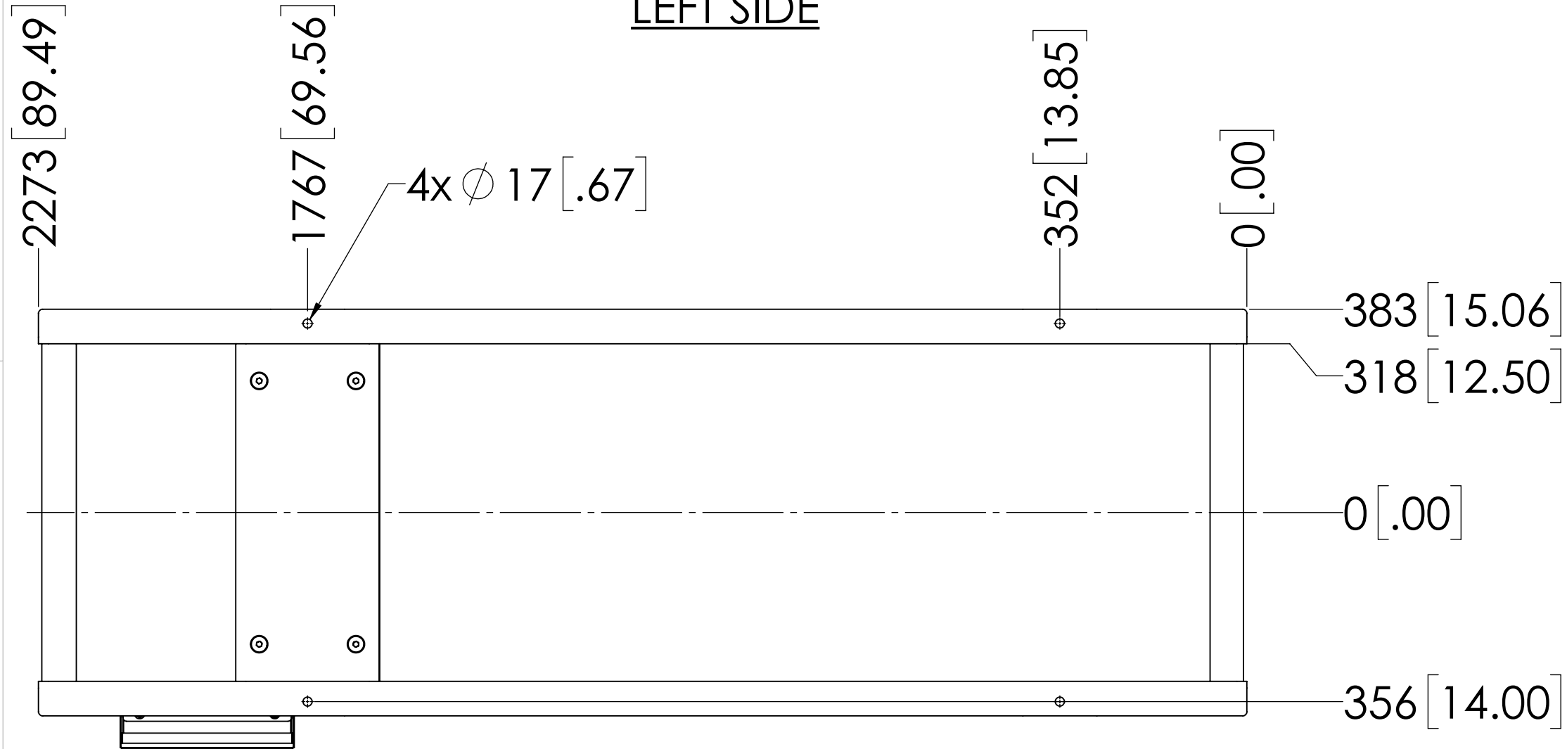
MOUNTING
