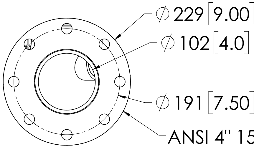
DETAIL A OPTIONAL DRY EXHAUST FLANGE SCALE 1 : 4
