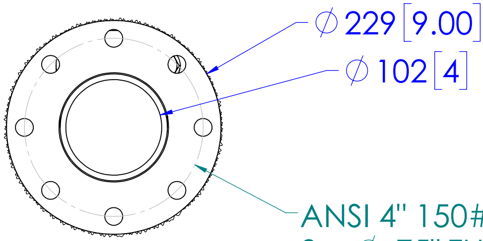
DETAIL A OPTIONAL DRY EXHAUST FLANGE SCALE 1 : 4
