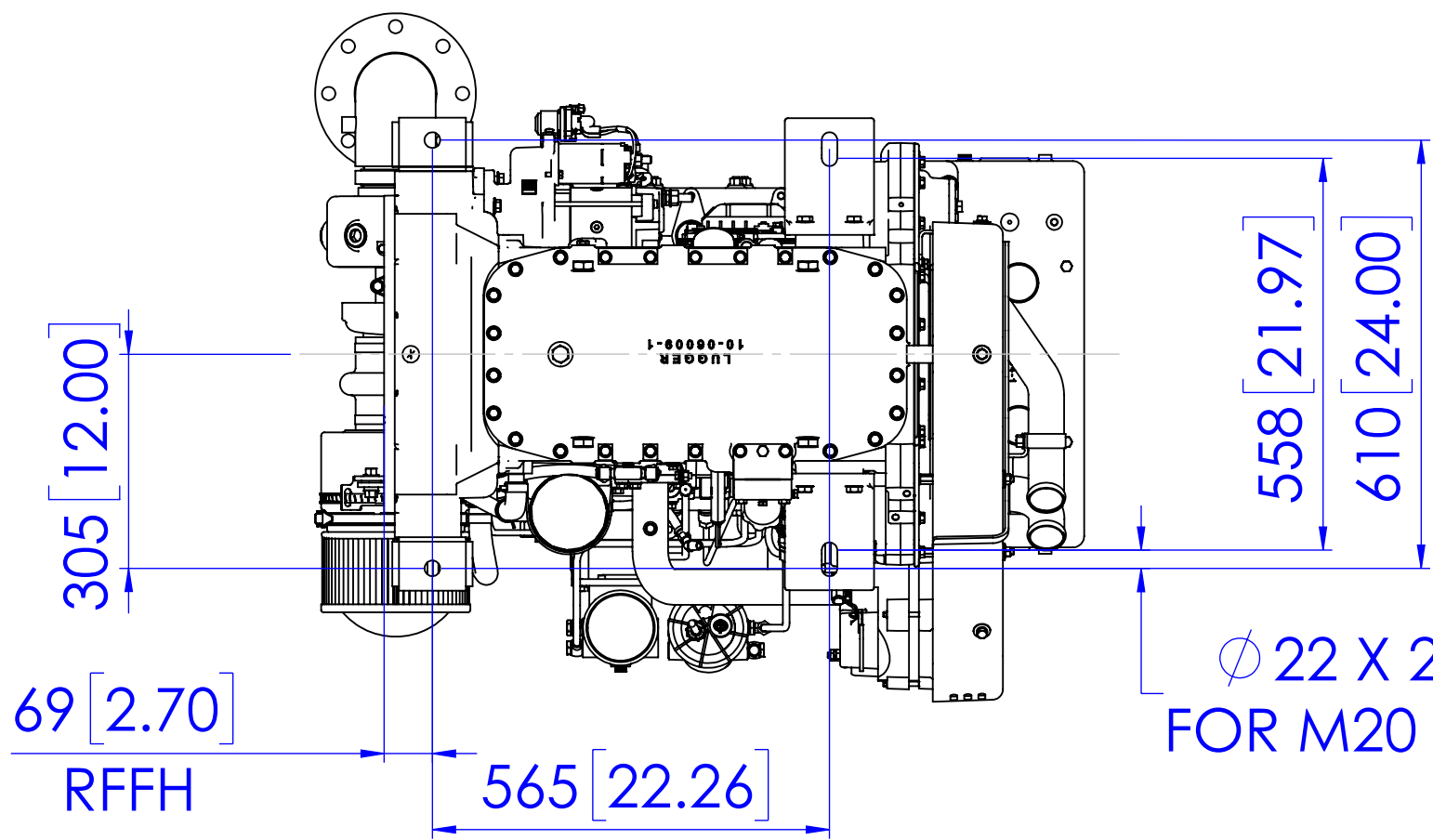
MOUNTING (W/O VIBRATION ISOLATION)
