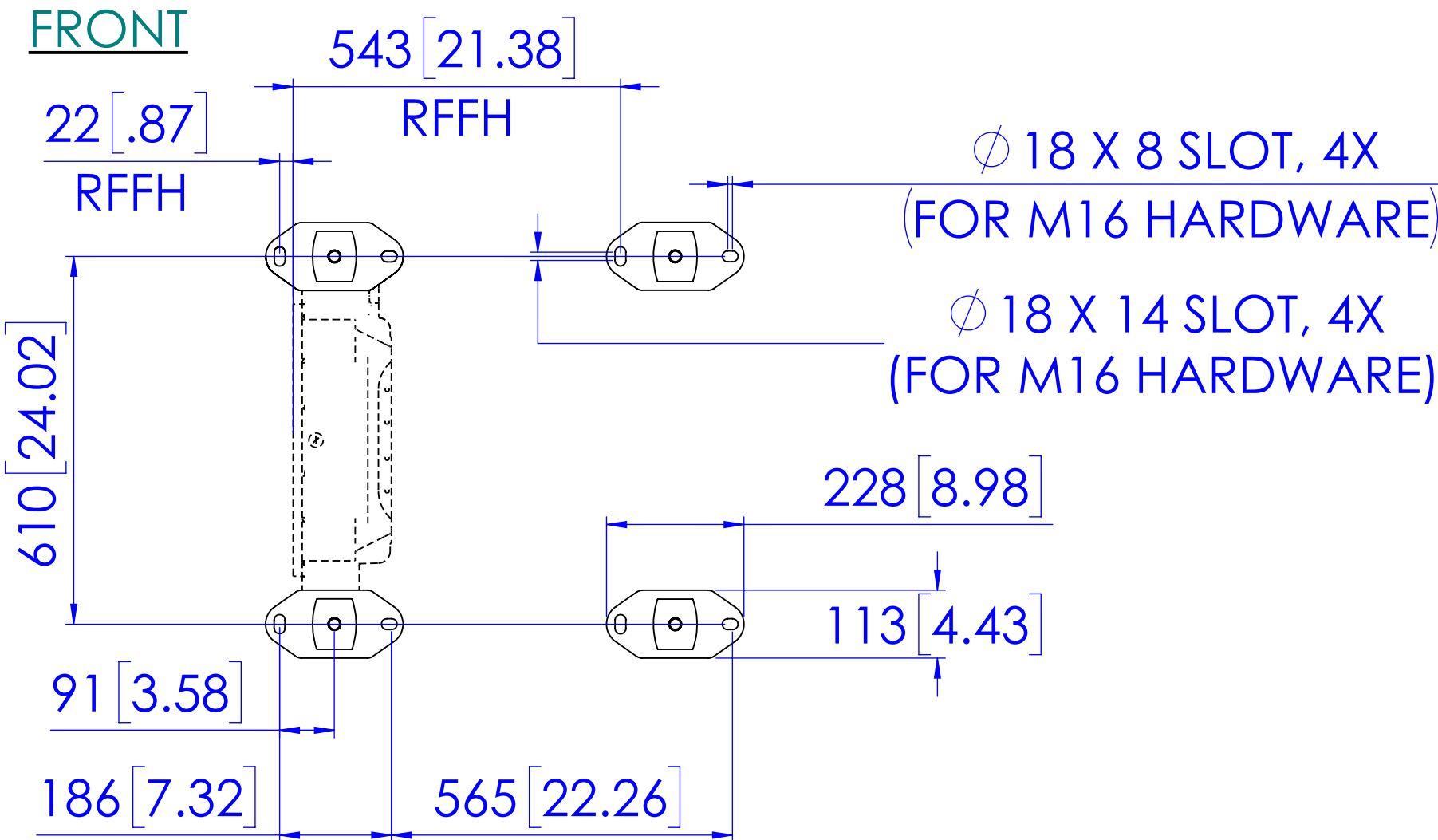
OPTIONAL VIBRATION ISOLATION FOOTPRINT
