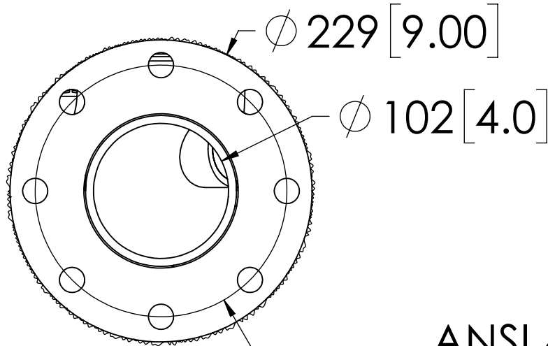
ANSI 4" 150# FLANGE 8x \varnothing 0.75" THRU HOLES ON 7.5" B.C. DETAIL A OPTIONAL DRY EXHAUST FLANGE SCALE 1 : 4
