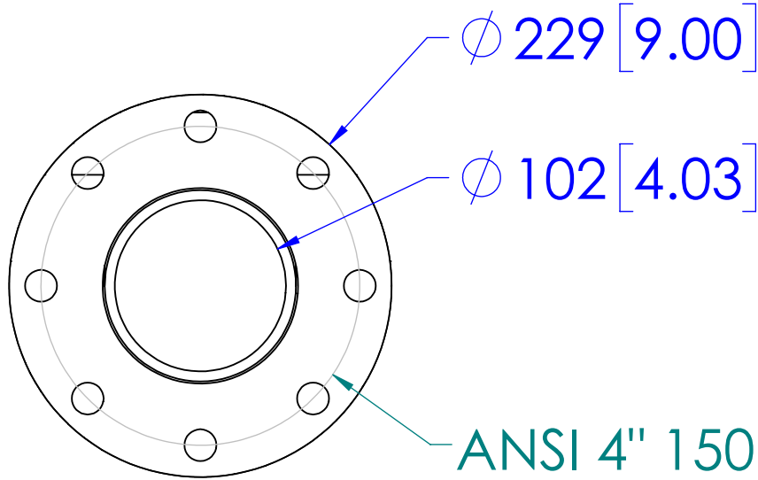
DETAIL A DRY EXHAUST FLANGE SCALE 1 : 4
