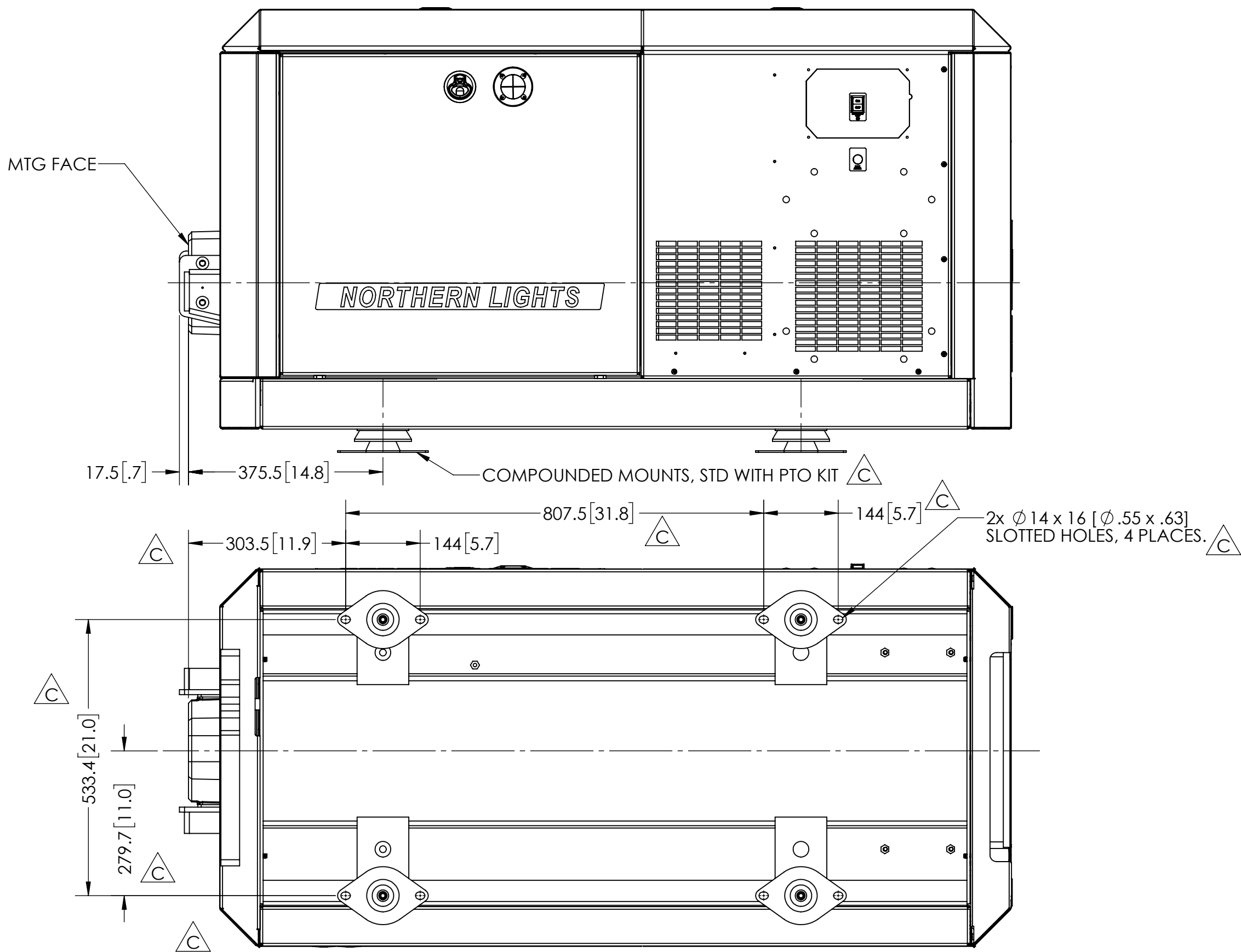
POWER TAKE OFF OPTION 06-61310
