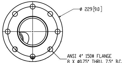
DETAIL A OPTIONAL DRY EXHAUST FLANGE SCALE 1 : 4
