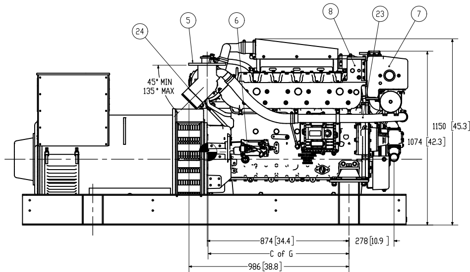
RIGHT VIEW
