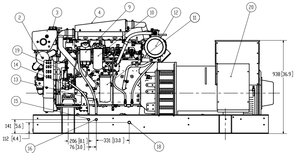
SERVICE SIDE (LEFT) VIEW
