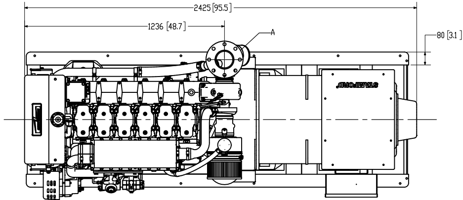
TOP VIEW
